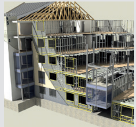
Building Information Modelling (BIM) is readily utilised in light steel framing
